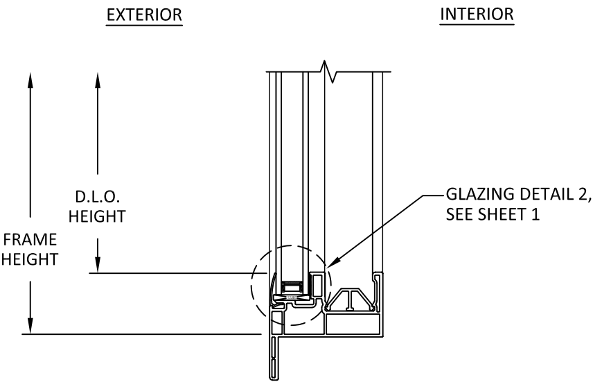
D 3 VERTICAL SECTION V152 FRAME - FX SILL
