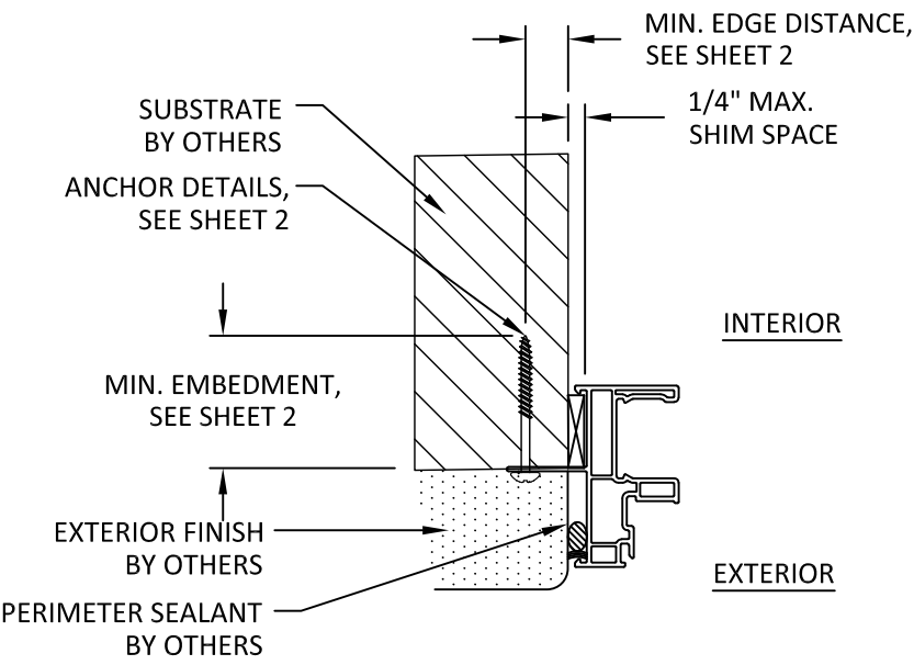
C 5 HORIZONTAL SECTION V100 FRAME NAIL FIN INSTALLATION
