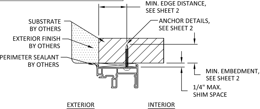
A 5 VERTICAL SECTION V142 FRAME THROUGH FRAME INSTALLATION
