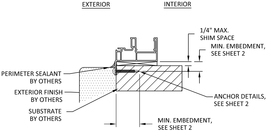
B 5 VERTICAL SECTION V101 FRAME NAIL FIN INSTALLATION
